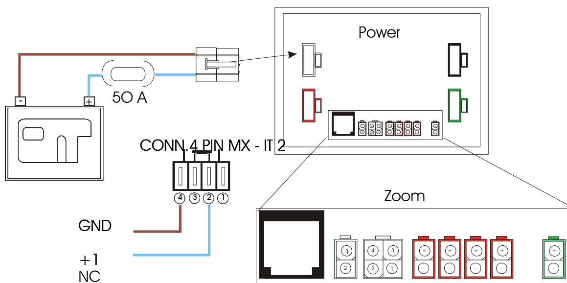
Figure 1 “Services Battery-Power Supply Unit Wiring”
