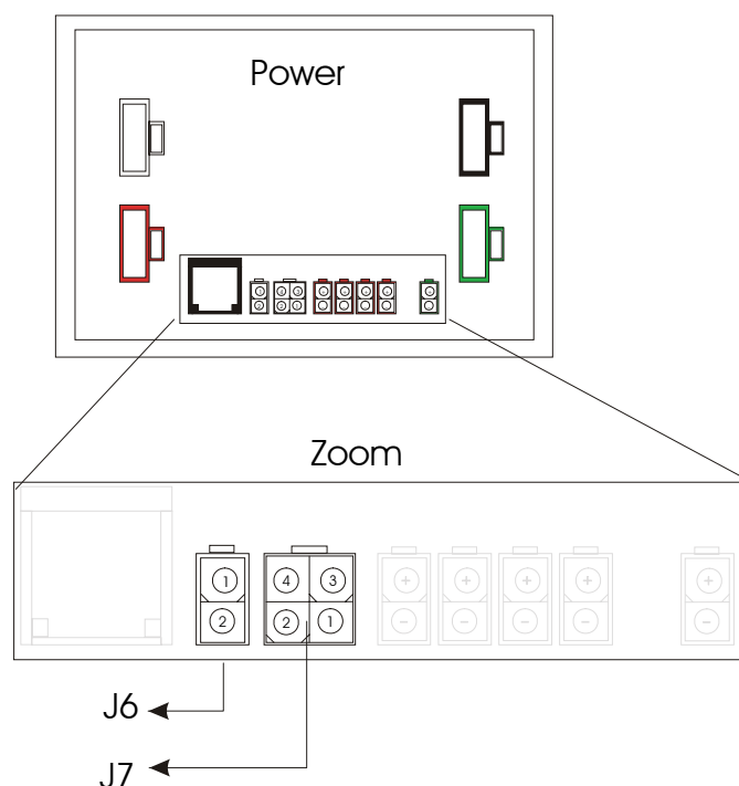
Figure 5"Power Supply Unit – Level Sensors Wiring"
